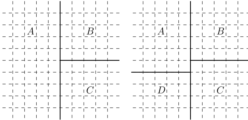
Fig. 2. On the left, illustration of the pattern used to prove the lemma 6. This always gives a resolving 3-partition of the space \mathbb{Z}^2 for gauges which do not contain vertical nor horizontal facet. On the right, the pattern used to prove the lemma 7. That pattern gives a resolving 4-partition for any convex distance in \mathbb{Z}^2 .
