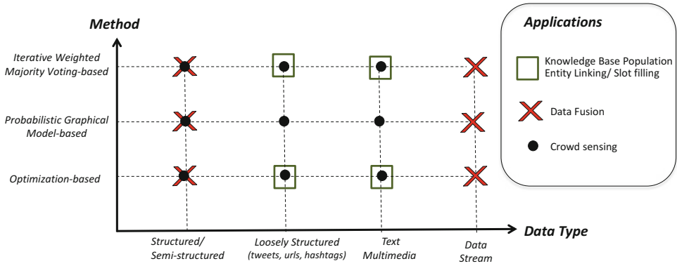
Truth Discovery, Fig. 1 Classification of the main approaches for truth discovery with typical application contexts, underlying computation model and data type
