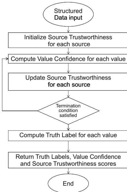
Truth Discovery, Fig. 4 Basic iterative algorithm for truth discovery
