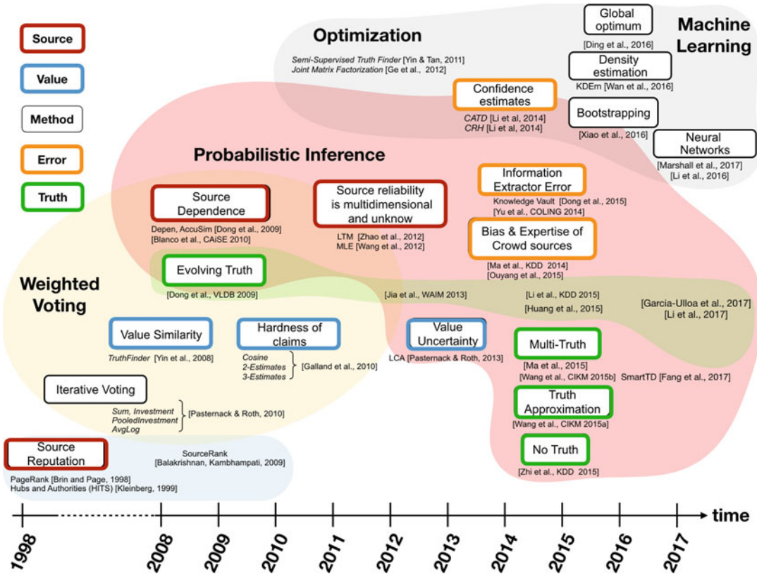
Truth Discovery, Fig. 3 Evolution of truth discovery research
