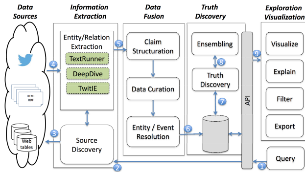
Figure 1: VERA Architecture
