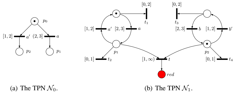
Fig. 1. Two TPNs exhibiting new discrete behaviors under infinitesimal perturbations.
