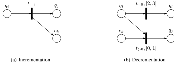
Fig. 2. Encoding instruction of a Minsky machine \mathcal{M} into a TPN \mathcal{N}_\mathcal{M} .
