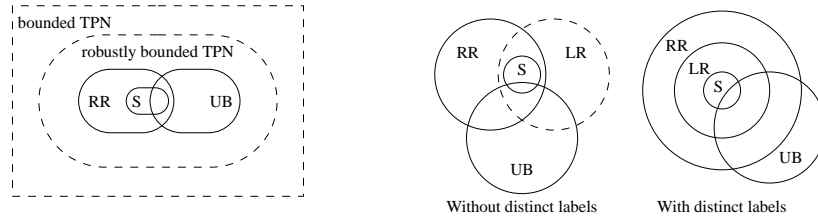
Fig. 5. RR stands for reach-robust, LR for language-robust, UB for bounded underlying PNs, S for sequential bounded TPNs. Dotted lines represent undecidable and solid lines decidable classes.
