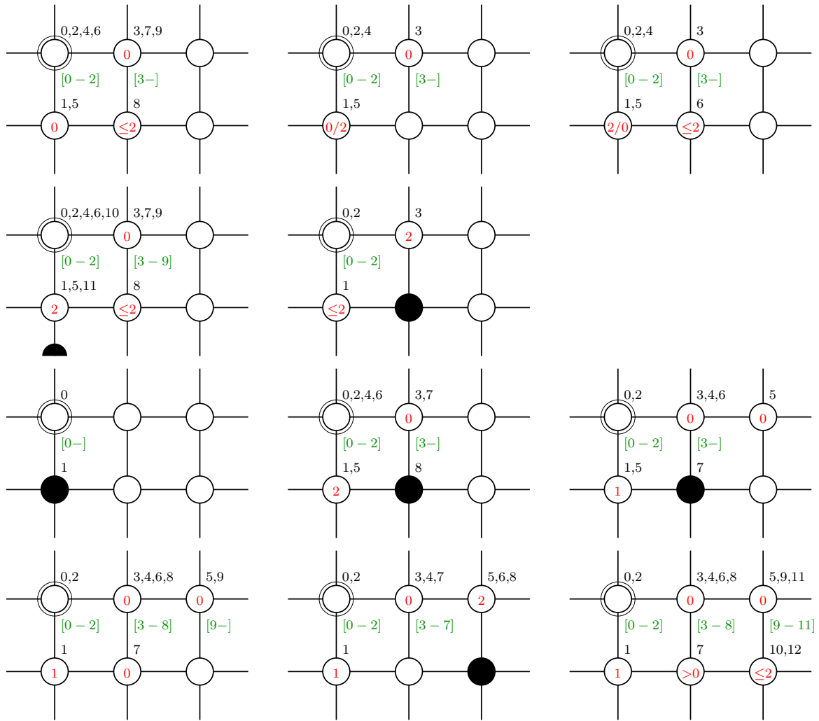
Fig. 1. The different trajectories an agent can follow while executing InitNextRing .
