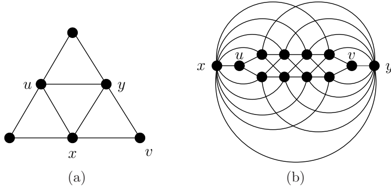
FIGURE 4. Two graphs in (a) CWW(k) \setminus CWR(k) , k \geq 2 and (b) CWW(4) \setminus CWW(5) .
