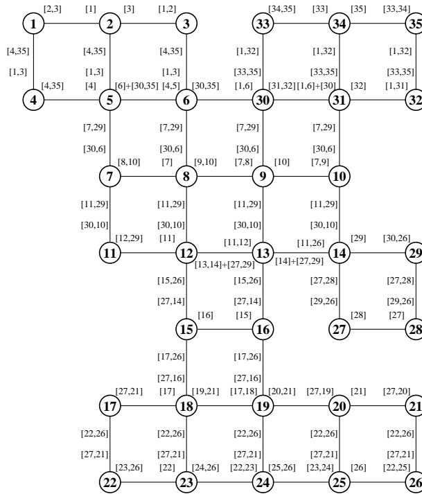
Fig. 8. A routing scheme in a rectilinear cell.
