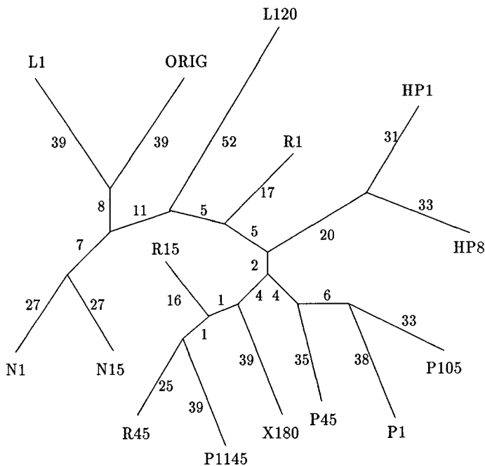
FIG. 3. A best l_\infty -approximation of \mathbf{d} in \mathcal{F}_{a,r}^m preserving the distances of ORIG.
