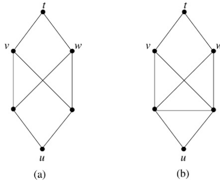
Fig. 2. Graphs fulfilling (Q) but not (Q!).
