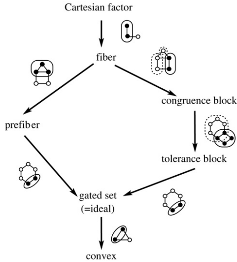
Fig. 6. Implications between fiber concepts.
