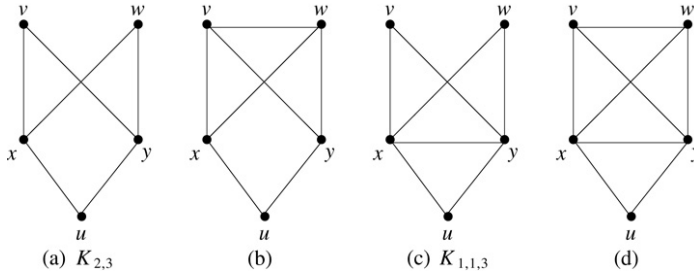
Fig. 1. Weakly modular graphs that are not weakly median.
