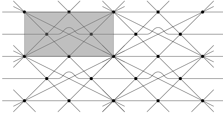
FIGURE 2. A non-stretchable line arrangement with an action of \mathbb{Z}^2 defined by letting a lattice basis act as translations by the two sides of the shaded rectangle. (The picture should be thought of as being repeated in vertical and horizontal direction). Any orientation of it gives rise to a FAOM. The quotient of the poset of covectors is the face category of a (pseudo)arrangement in the 2-dimensional torus (e.g., obtained by identifying opposite sides of the shaded rectangle), whose cells are counted by the Tutte polynomial of the group action on the underlying semimatroid.
